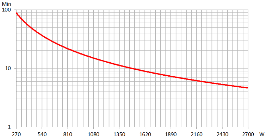
Figure 18 – Runtime graph of SMALLT3A10
