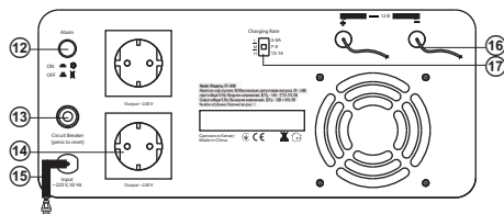
Fig. 4. Rear panel of RT-800*
